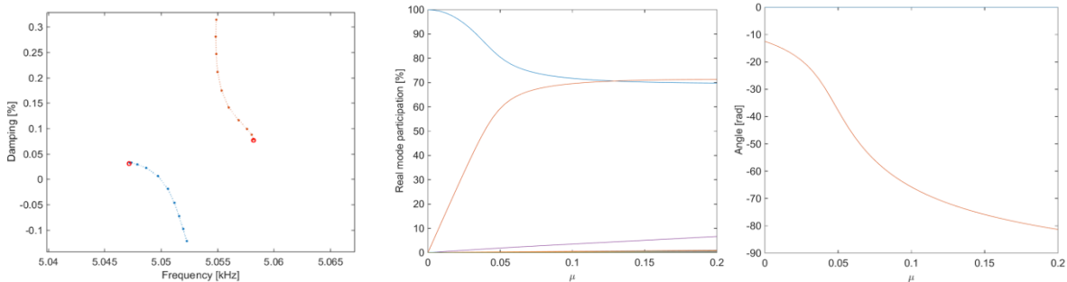
Figure 3 : Evolution of complex modes with the friction coefficient: roots (left), real mode participation to the complex mode #8 (middle) and phase between real modes #8 and #9 (right)
