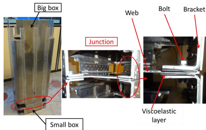
Figure 1 : Fuselage testbed 1155×409×259mm
